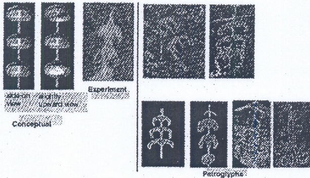
Fig. 29. (Left) Vortex formation in sub and multimegampere pinched plasma columns. (Right) Petroglyphs.
