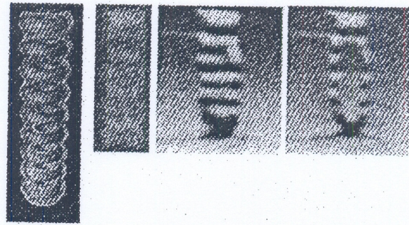
Fig. 8. Inner toroids within the stack of spheroids produced in a multimegaampere plasma column. (a) Basic geometry. (b) Centimeter-size 1.3-MA pinch. (c) Centimeter-size 6-MA pinch. (d) Centimeter-size 6-MA pinch with optically dense (brightest) plasma shown.
