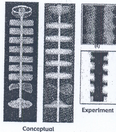
Fig. 9. (Left) Illustrations of simulations of the flattening of a stack of multimegaampere conducting plasma toroids. The current causes the toroids to both flatten out in the center and start to wapp and fold at the ends as shown. (Right) X-ray radiograph of a 16-MA pinched plasma 4 cm in diameter. (Top) Plasma sinusoidal pinch perturbation at 6.5 \mu s. (Bottom) Formation of flattened toroids from the initial ripples at 9.5 \mu s. The bottom figure rungs appear cutoff, but are the natural shape. (Los Alamos Plasma Physics, P-24).
